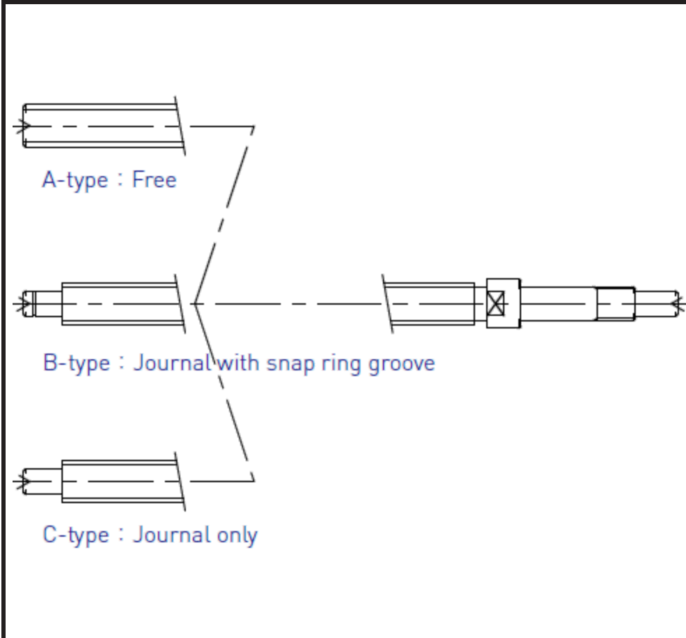
Fig. A-22 : Shaft supported end profile
