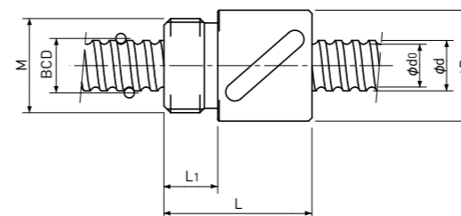
Type-2:Return-tube type
